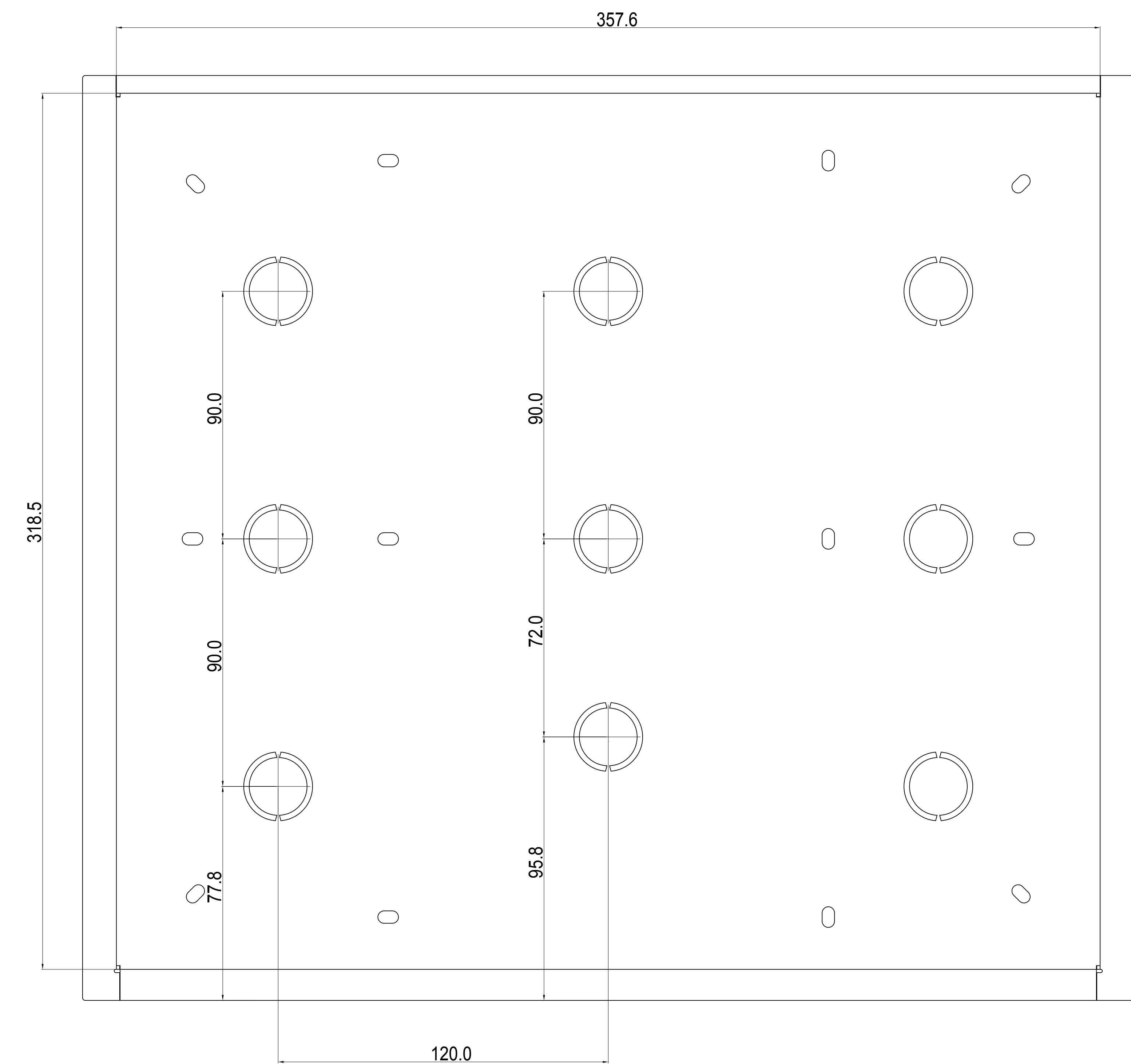
4 BACK VIEW
