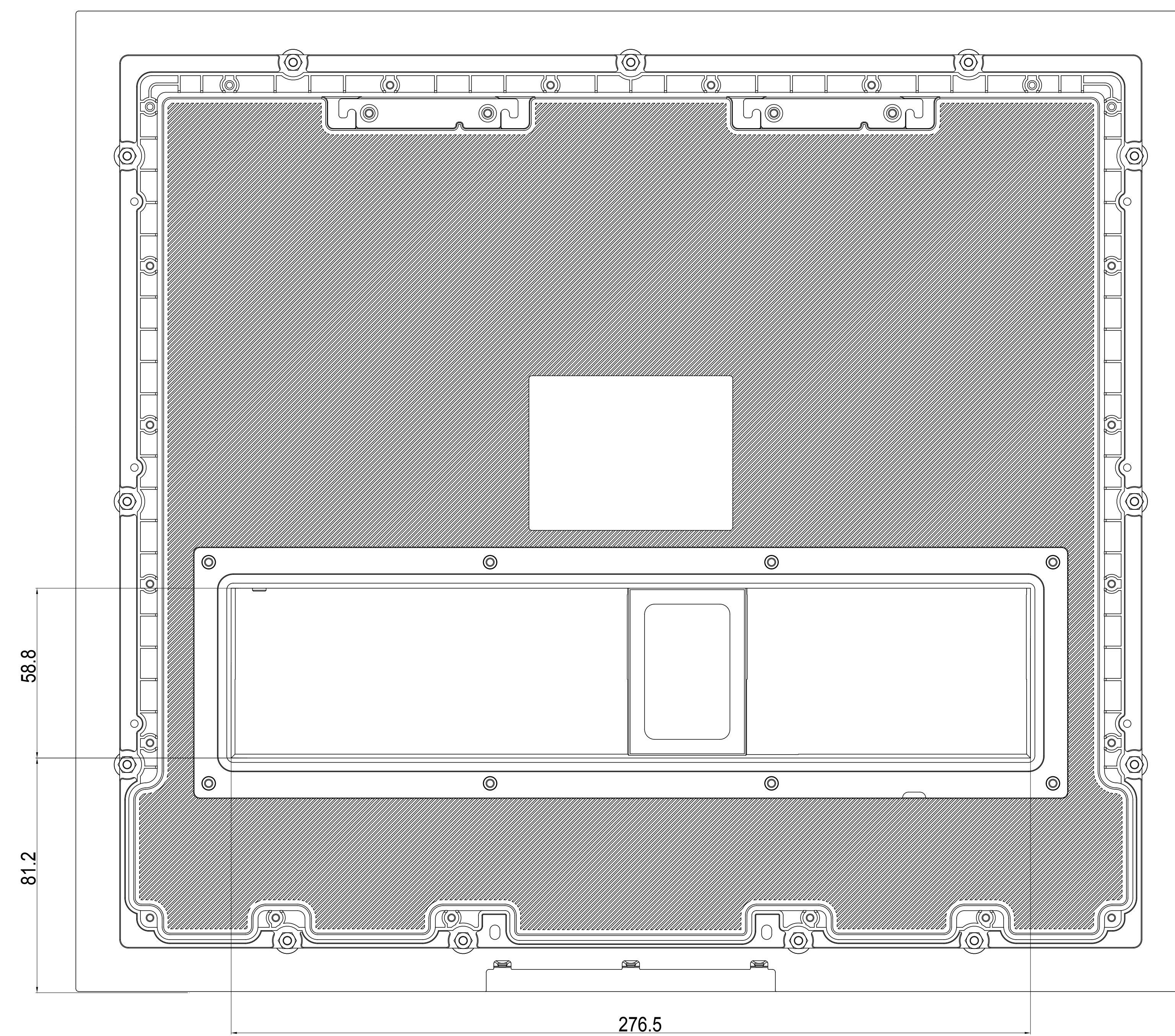
4 BACK VIEW
