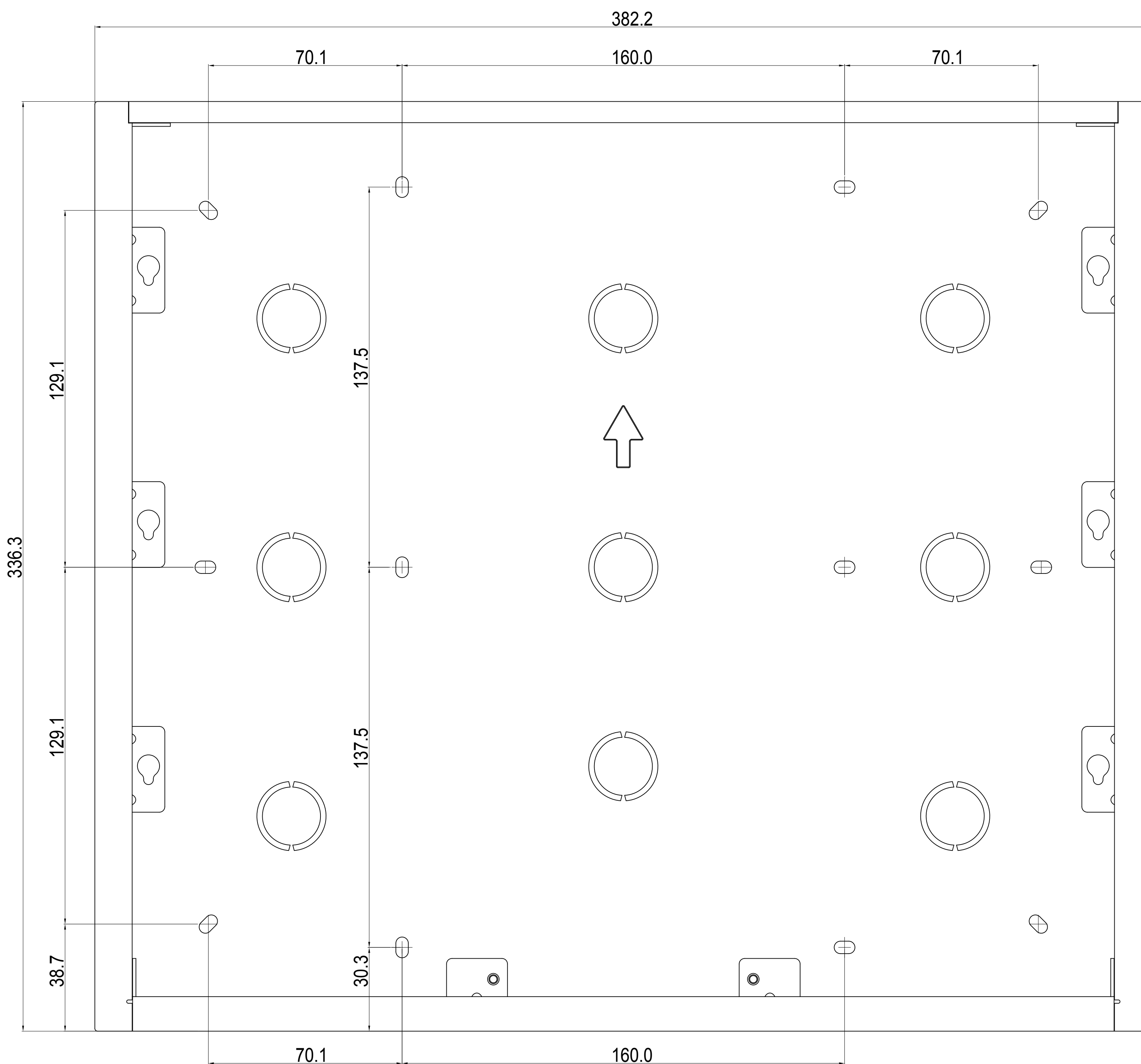
1 FRONT VIEW
