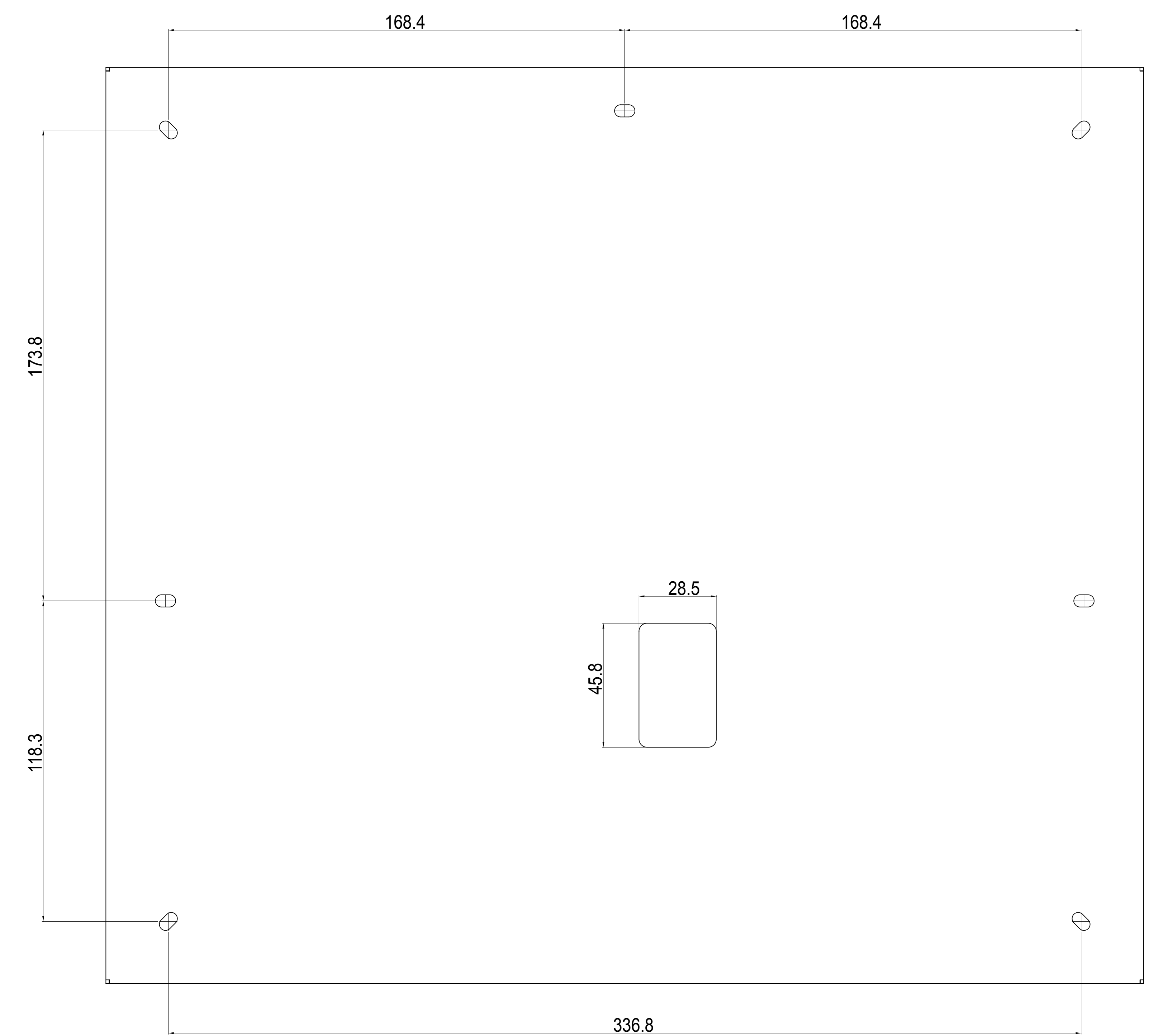
4 BACK VIEW
