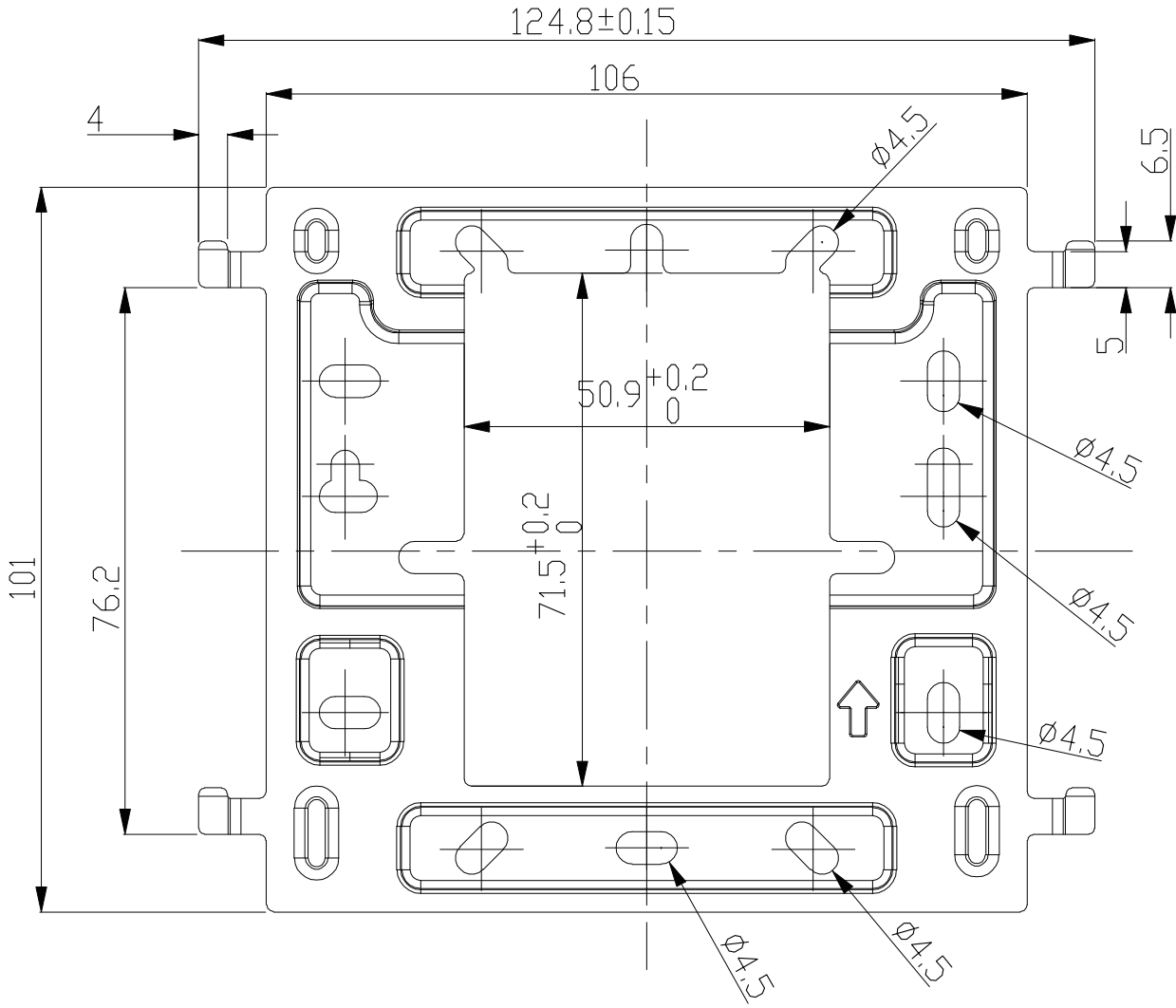
Wall-mounting template(mm)
