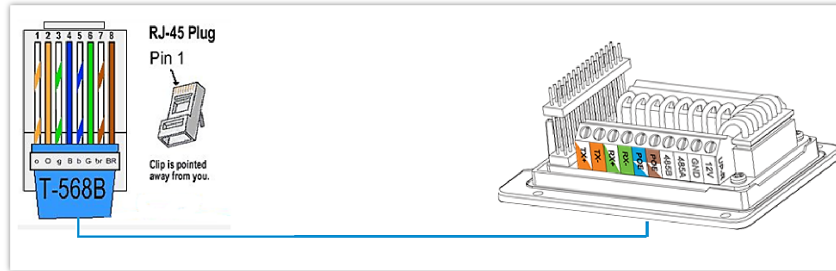
Connection Example
