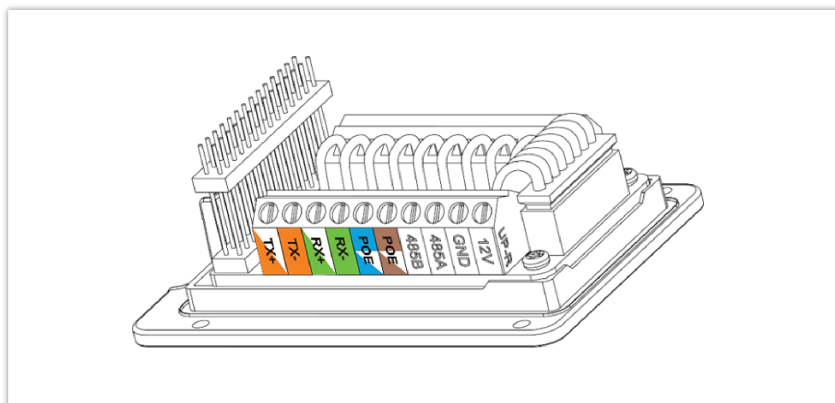
GDS370x Back Cover
