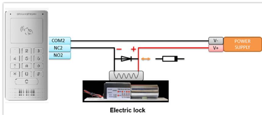
Protection Diode – Example 2
