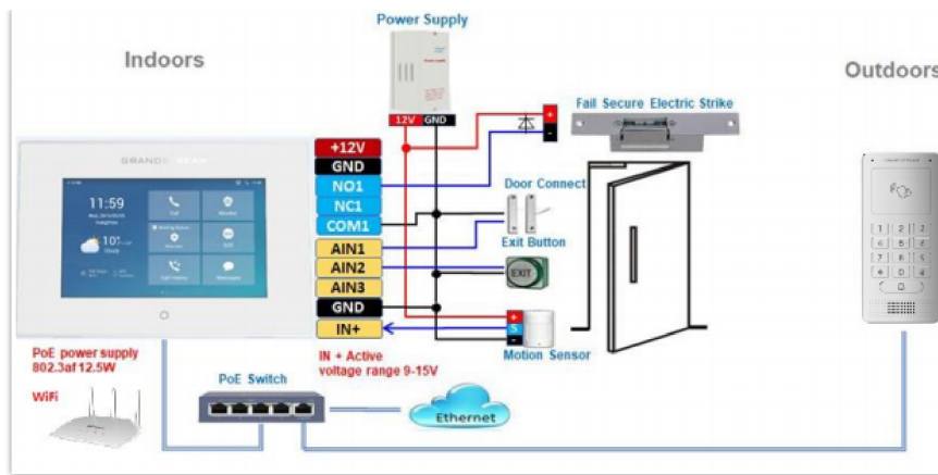
GSC3570 secure open door via GDS3705
