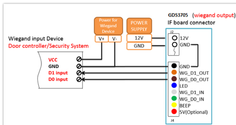
Wiegand Output Wiring Example
