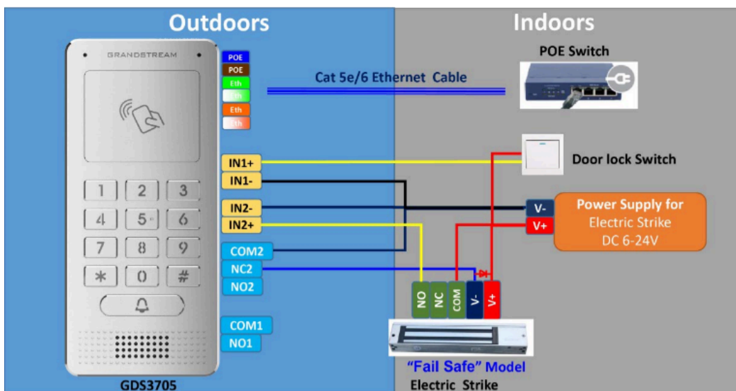
Wiring Sample using PoE to power GDS370x and 3 rd party Power Supply for Electric Strike
