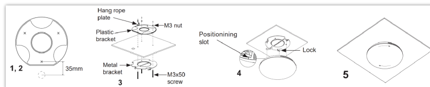
Ceiling Mount
