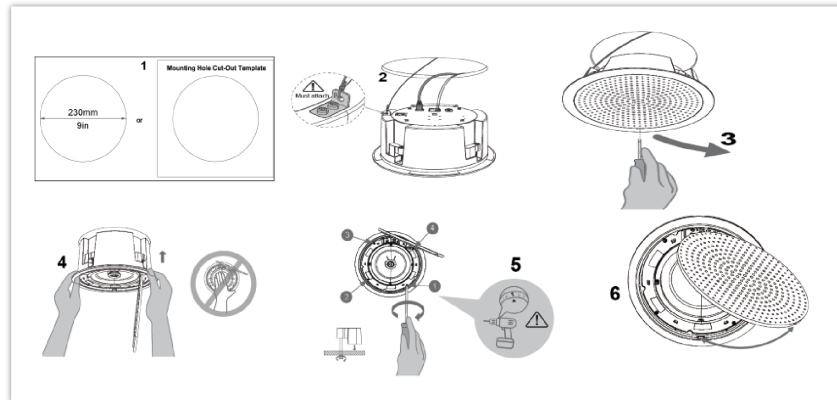
Ceiling Mount
