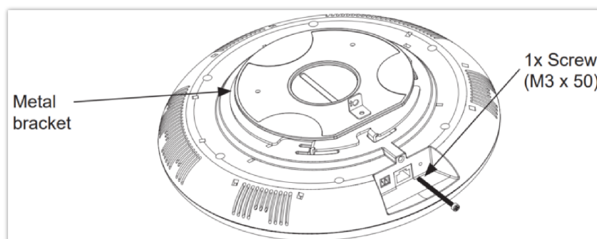
Anti-theft Installation
