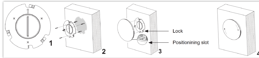
Wall Mount
