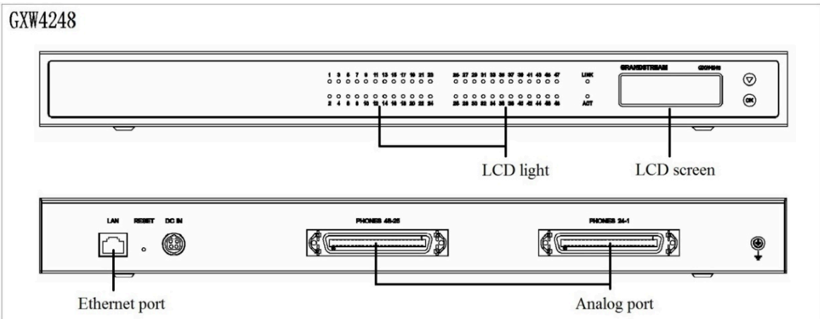
Diagram of GXW4216/24/32/48 Panel
