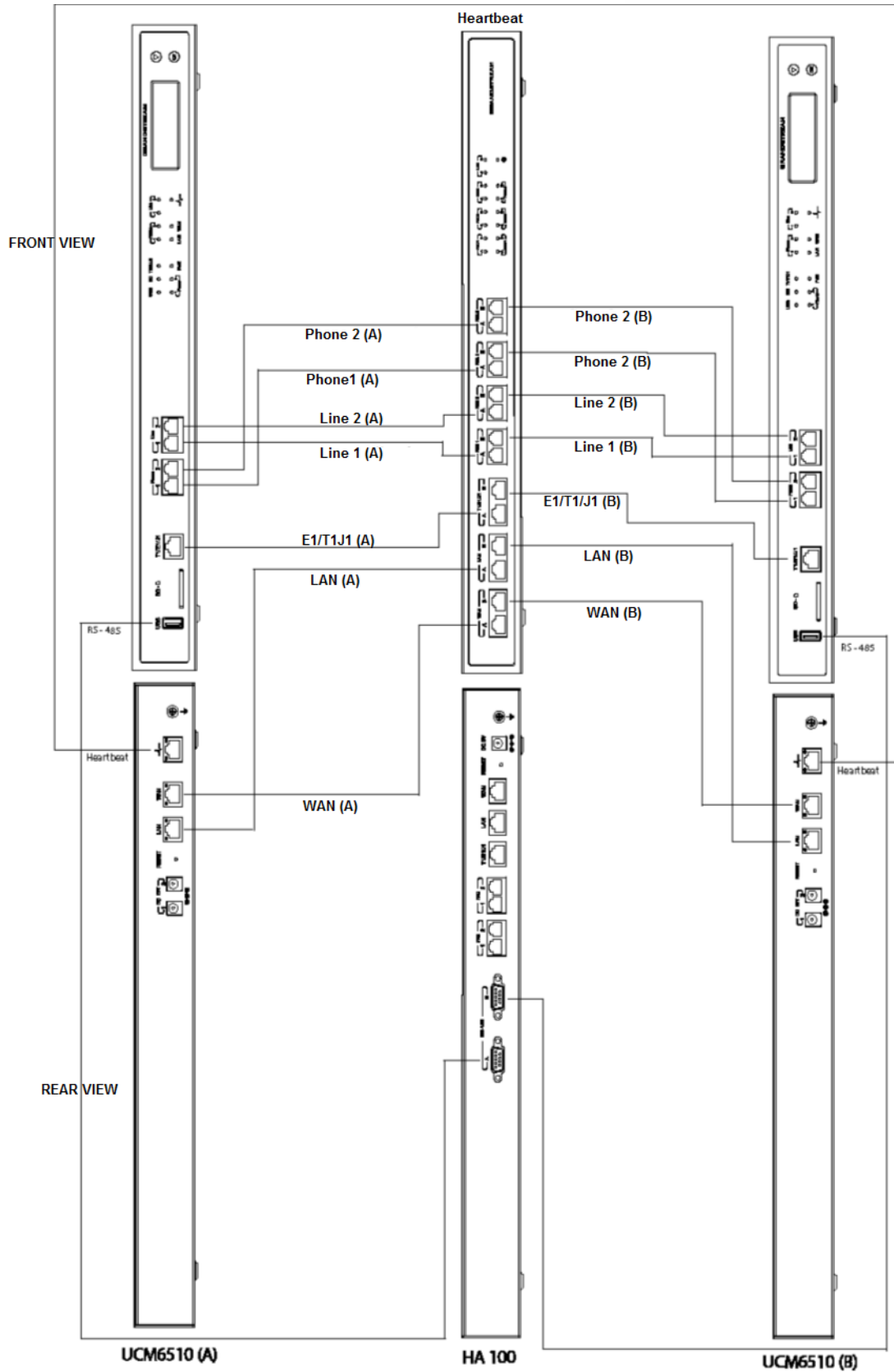
Figure 3: HA100 Connection with UCM A and UCM B
