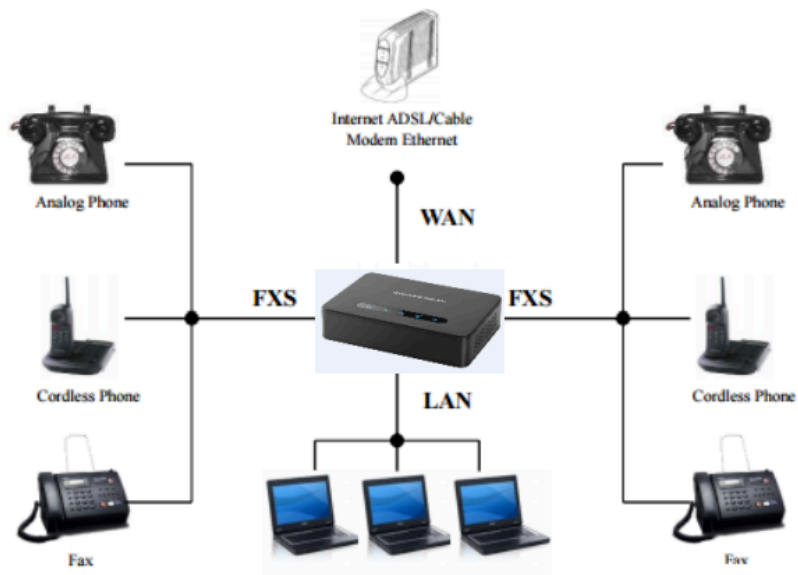
Connecting the HT812/HT814
