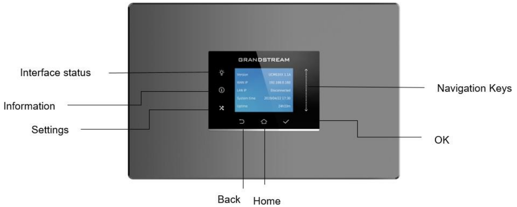
UCM6301 Top View
