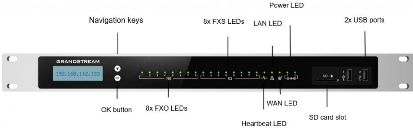
UCM6308 Front View
