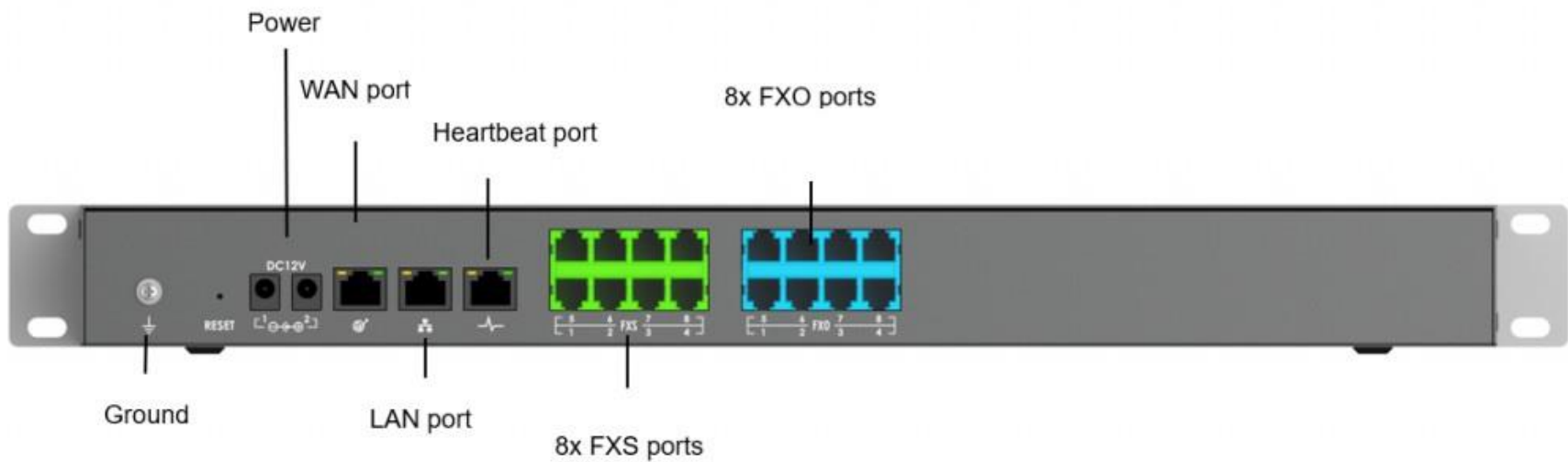
UCM6308 Back View
