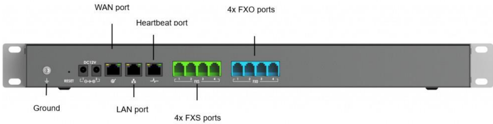
UCM6304 Back View
