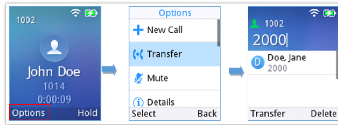
Figure 39: Blind Transfer
