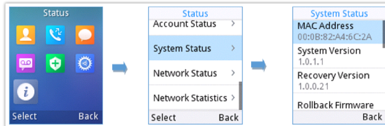
Figure 22: System Status
