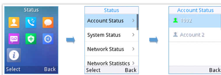
Figure 20: Account Status
