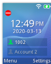
Figure 37: DND Enabled
