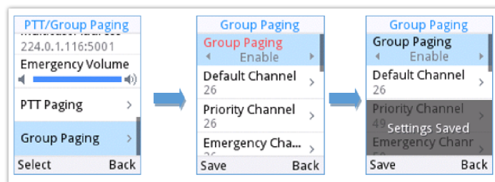
Figure 60: Group Paging
