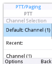
Figure 57: PPT Channel
